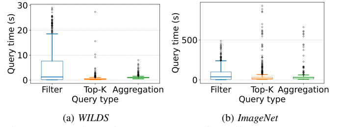
Fig. 7: Query time of MASKSEARCH for different query types. Index size for MASKSEARCH: \sim 5\% of dataset size.
