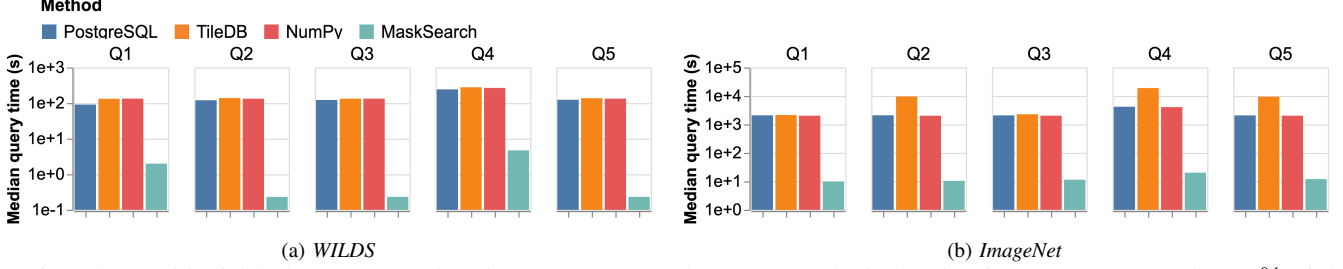
Fig. 6: End-to-end individual query execution time on WILDS and ImageNet . The index size for MASKSEARCH is \sim 5\% of the original compressed dataset size for both datasets. Note the log scale on the y-axis.
