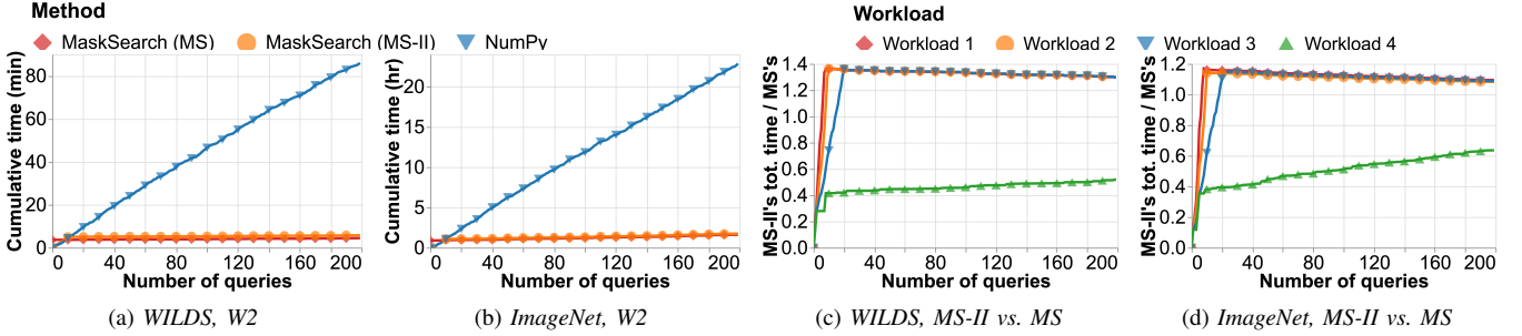
Fig. 10: Cumulative total time, incl. index building time and query time, for multi-query workloads. MS-II and MS refer to MASKSEARCH w/ and w/o incremental indexing, respectively. (a) and (b) show the total time for MS, MS-II, and NumPy for Workload 2; (c) and (d) show the ratio of the cumulative total time of MS-II to that of MS for all workloads. The index size for MS is \sim 5\% of the corresponding dataset. MS-II builds the index incrementally using the same index configuration as MS.
