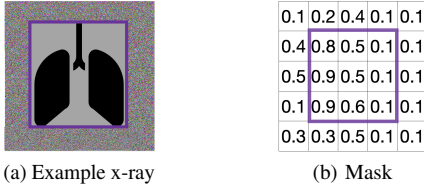
Fig. 3: A toy image motivated by [15] and its mask. The purple box is the ROI. Predicates on masks often involve counting the number of pixels in the ROI with values in a range, e.g., # pixels in the ROI with values in (0.85, 1.0) is 2.
