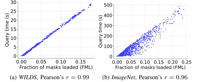
Fig. 8: Relationship between end-to-end query time and the fraction of masks loaded (FML) for a query. (a) WILDS , Pearson’s r = 0.99 (b) ImageNet , Pearson’s r = 0.96
