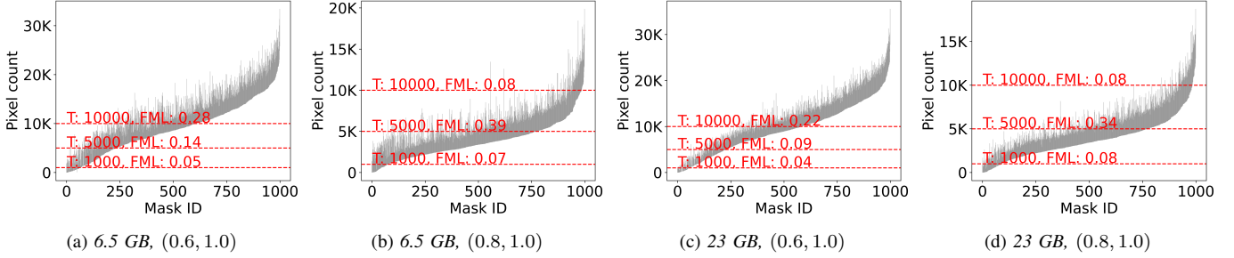
Fig. 9: Distribution of bounds for ImageNet masks computed by MASKSEARCH. Each subfigure represents a combination of (index size, (lv, uv) ). Each vertical segment represents the lower and upper bounds of \text{CP}(\text{mask}, \text{roi}, (lv, uv)) for a single mask. FML is the fraction of masks loaded by MASKSEARCH given a predicate \text{CP}(\text{mask}, \text{roi}, (lv, uv)) > T , which is equal to the fraction of the vertical segments that intersect with the horizontal dashed line defined by T .
